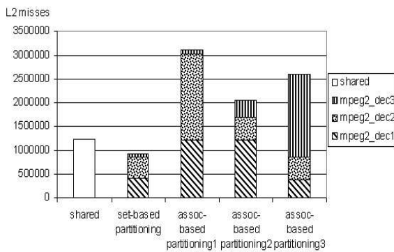
Fig. 5. Cache misses for different partition types - example 2
