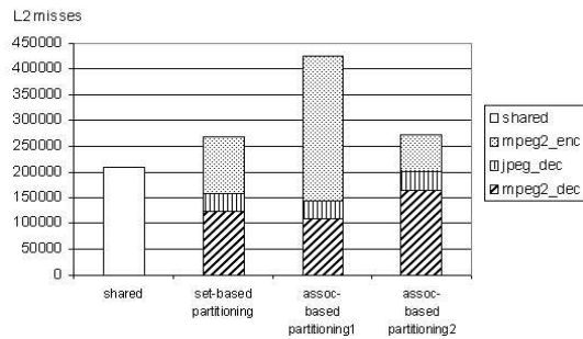
Fig. 6. Cache misses for different partition types - example 3
